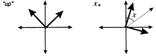
Fig. 1. Interpretation of the spin “up” and \chi_+ states in terms of the hidden polarization angle \alpha . The thick arrows represent equally probable directions.
