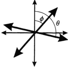
Fig. 6. “Unbiased” HV_3 representation of the hidden variables distribution for the singlet state
