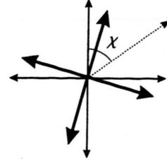
Fig. 3. Interpretation of the singlet distribution for \alpha when the singlet is parameterized in terms of the angle \chi .
